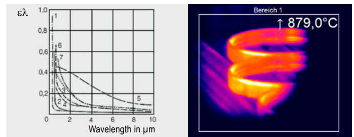
Spectral emissivity of metals: 1 Silver, 2 Gold, 3 Platinum, 4 Rhodium, 5 Chrome, 6 Tantalum, 7 Molybdenum
