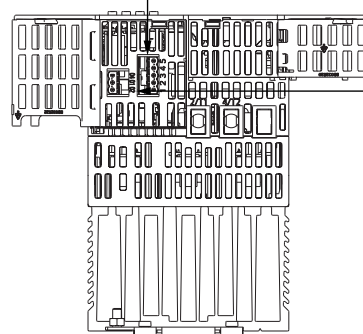
View on lower face
