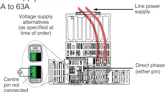
View on upper face 63 unit shown; 32A unit is similar
