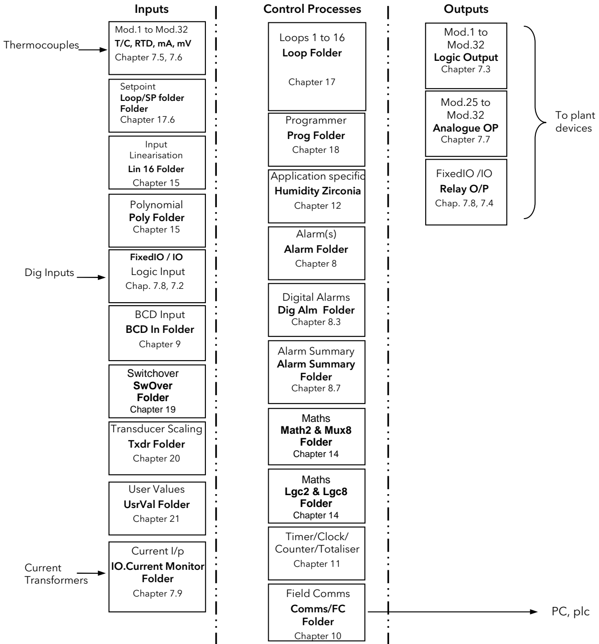
Figure 4-1: Controller Example
