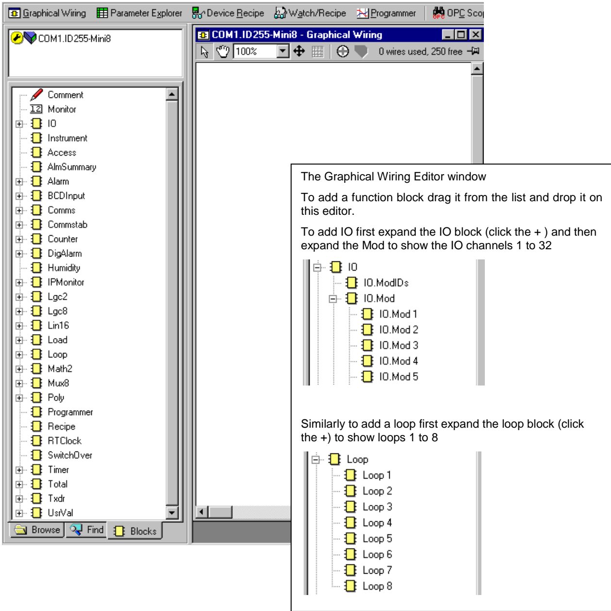
Figure 3-8: List of Function Blocks & Graphical Wiring Window
