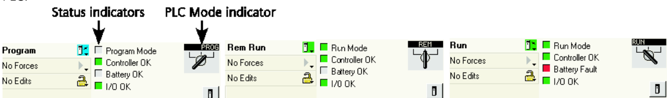
Figure 10-18: Status Indicators
