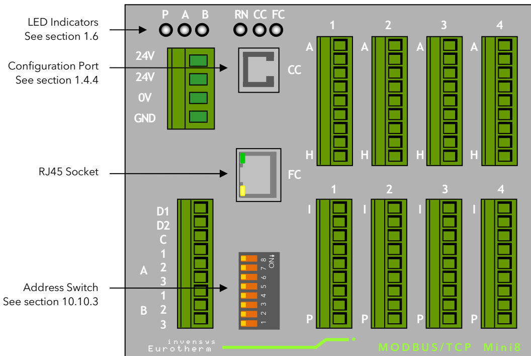
Figure 1-10: EtherNet TCP Front Panel Layout
