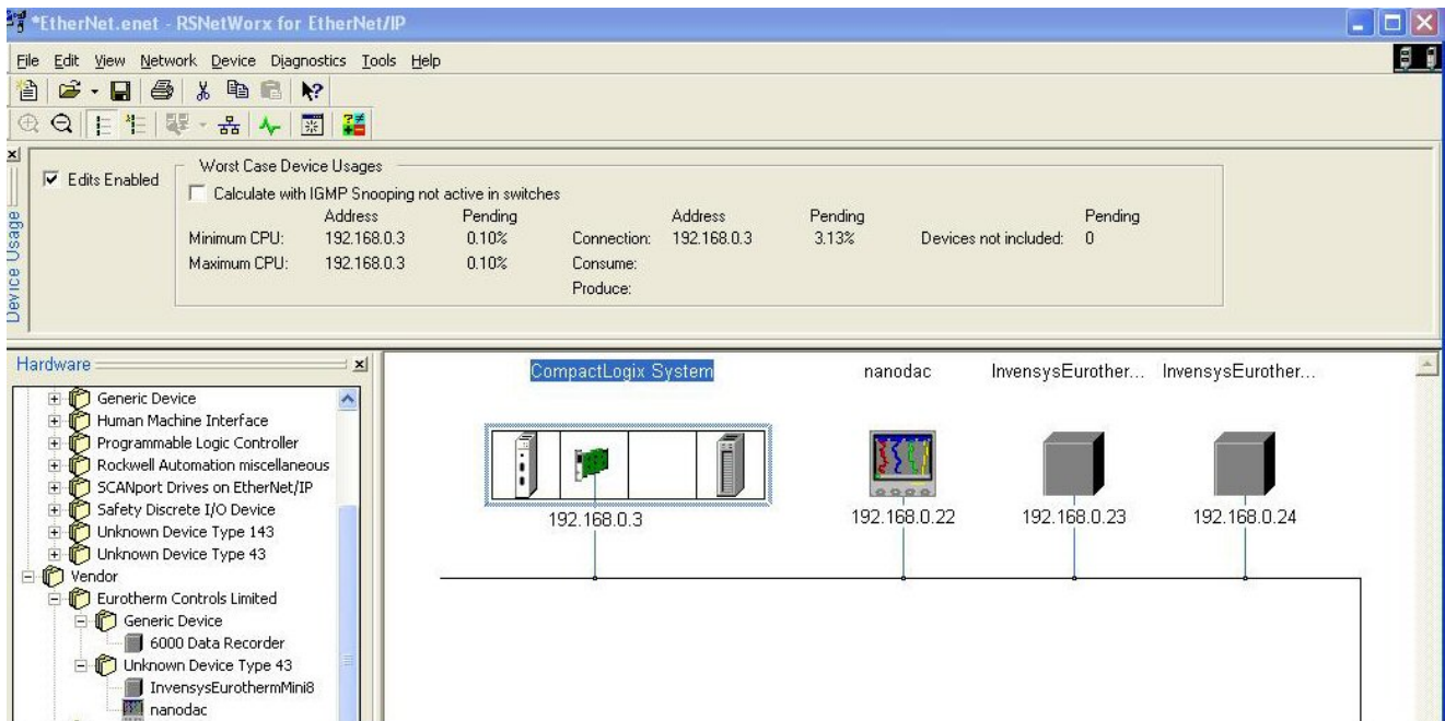
Figure 10-19: Example of Eurotherm Products on an EtherNet/IP Network
