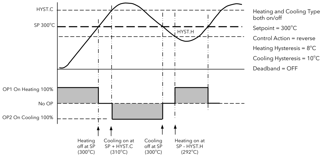
Figure 17-16: Deadband OFF
