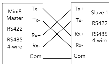
Figure 1-6: Rx/Tx Connections for RS422, RS485 4-wire
