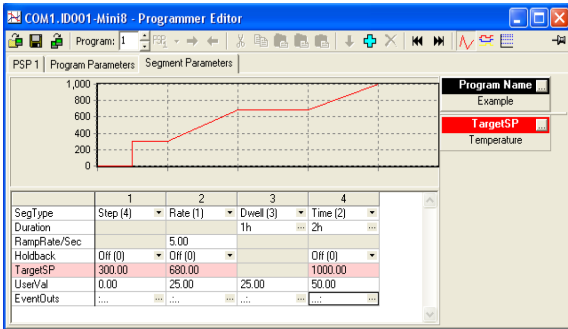
Figure 18-5: Spreadsheet Editor with 4 different segment types
