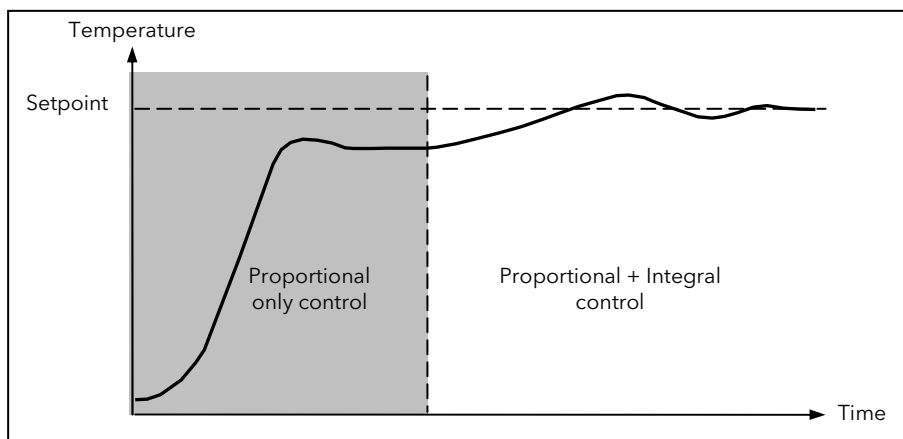
Figure 17-3: Proportional + Integral Control
