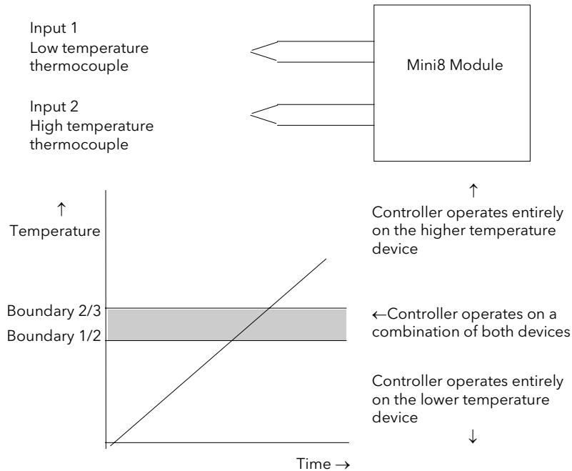
Figure 19-1: Thermocouple to Pyrometer Switching
