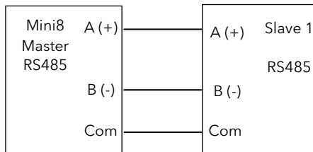
Figure 1-5: Rx/Tx Connections RS485 2-wire
