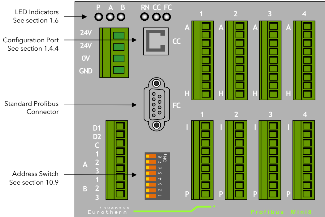
Figure 1-9: Profibus Panel Layout - Standard D Connector
