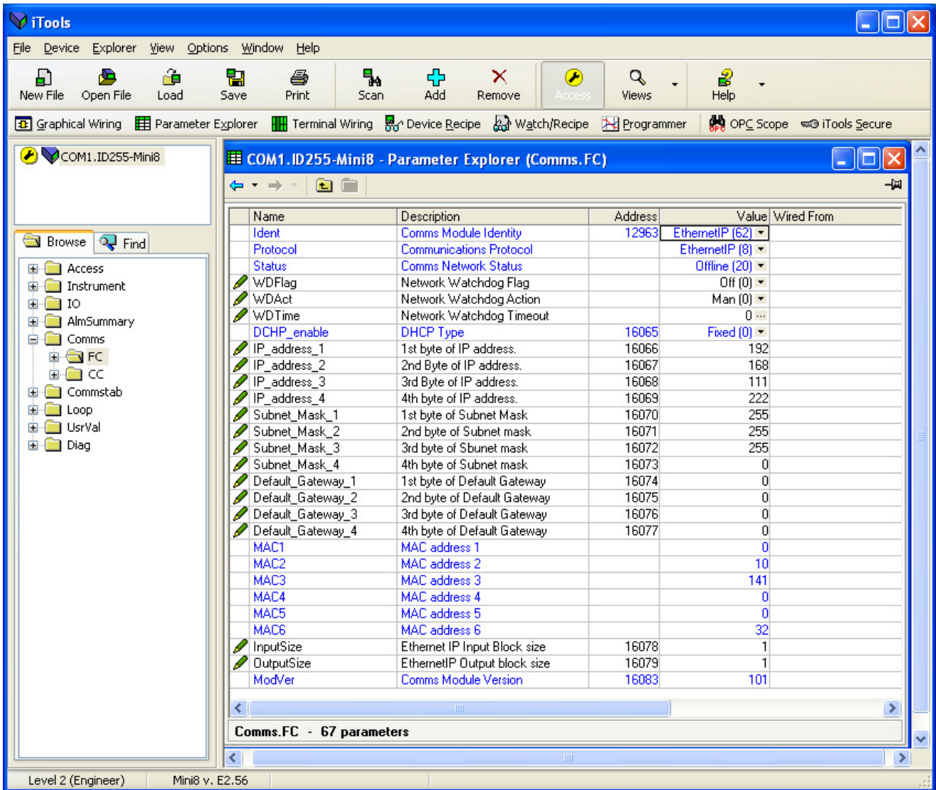
Figure 10-2: EtherNet/IP Parameters
