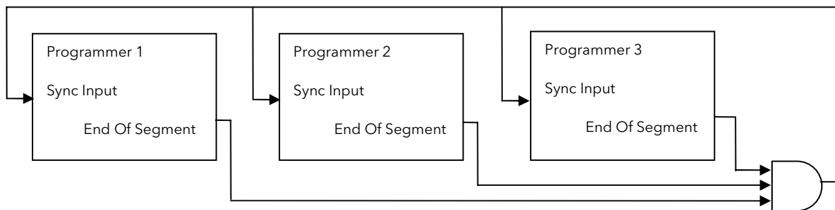
Figure 18-10: Synchronisation of programmer blocks
