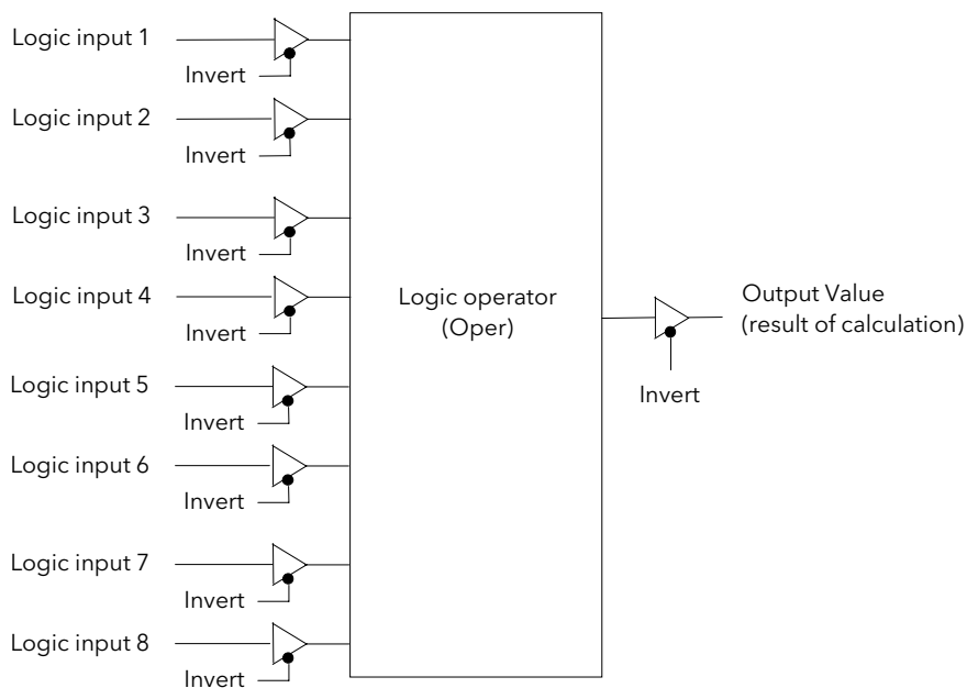
Figure 14-2: 8 Input Logic Operators
