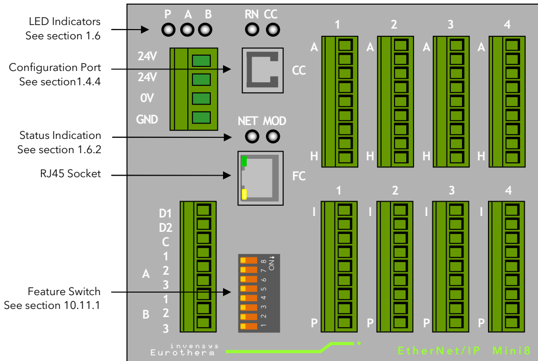
Figure 1-11: EtherNet/IP Front Panel Layout
