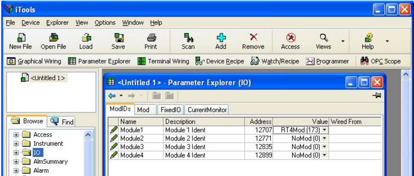
Figure 3-6: Mini8 Controller IO Module1 Defined as RTD
