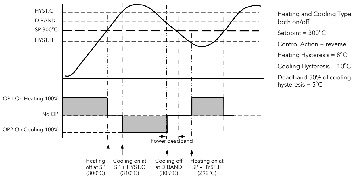
Figure 17-17: Deadband ON set at 50% of Cooling. Hysteresis = 5°C
