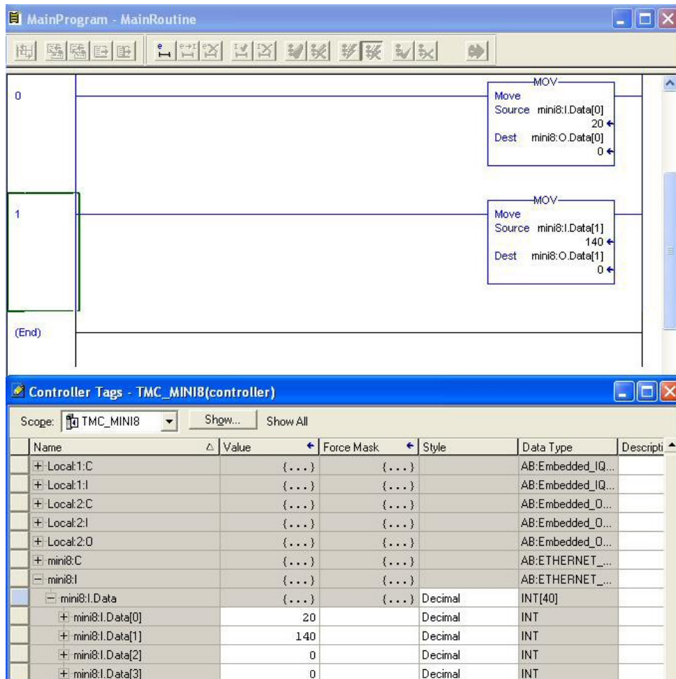
Figure 10-17: Monitor Inputs and Outputs via Controller Tags
