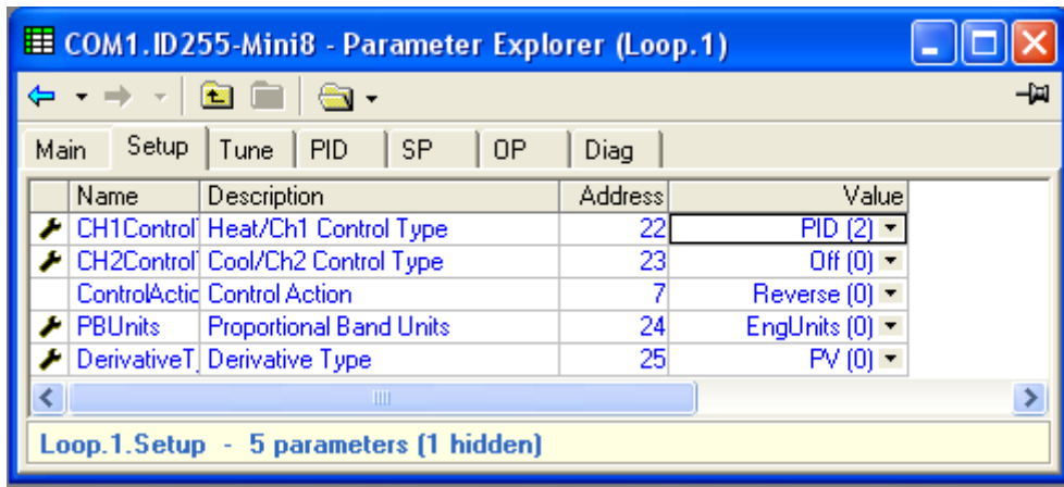
Figure 3-10: PID Function Block
