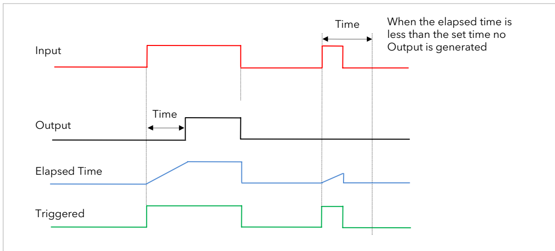
Figure 11-5: On Delay Timer under Different Input Conditions
