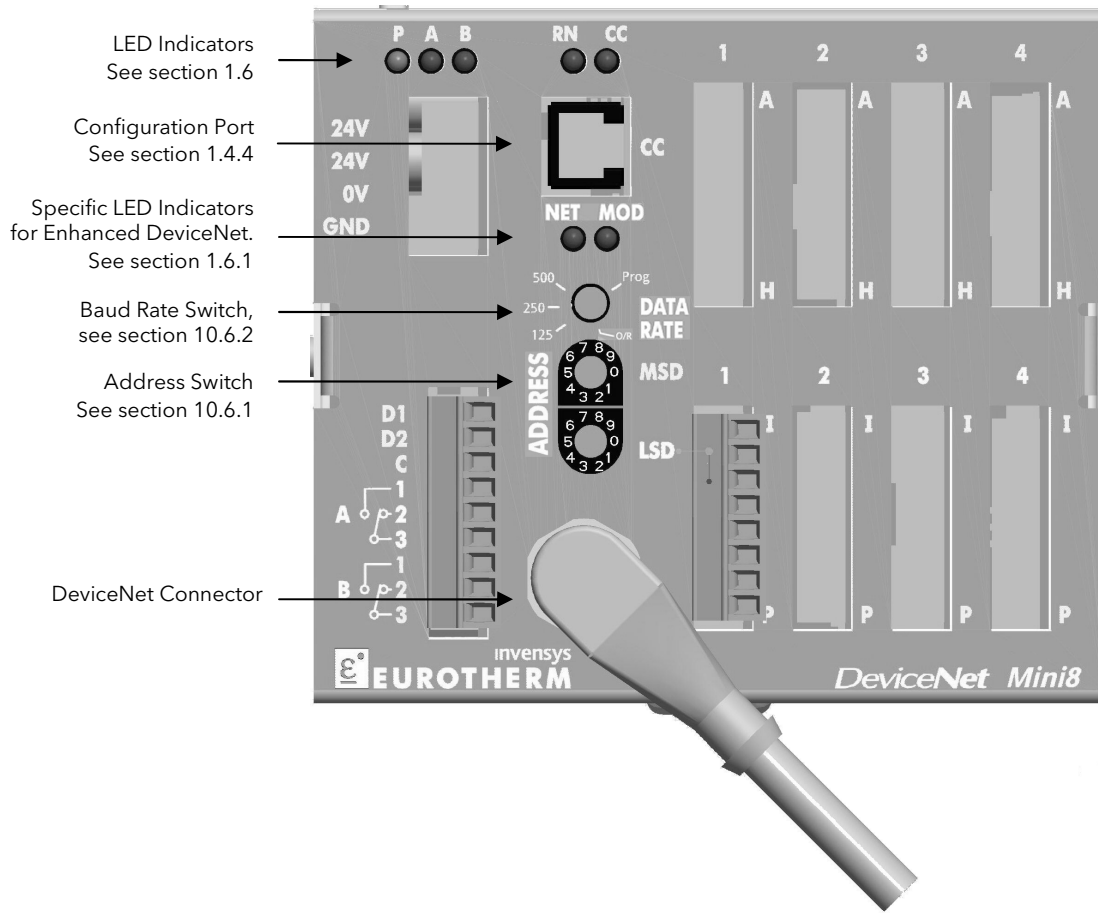
Figure 1-8: Enhanced DeiceNet Panel Layout
