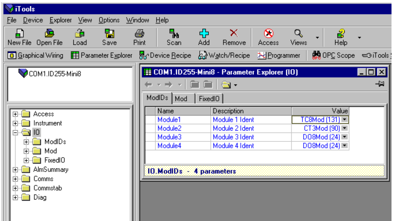
Figure 3-3: Mini8 controller I/O Modules
