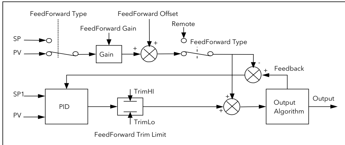
Figure 17-15: Implementation of Feedforward
