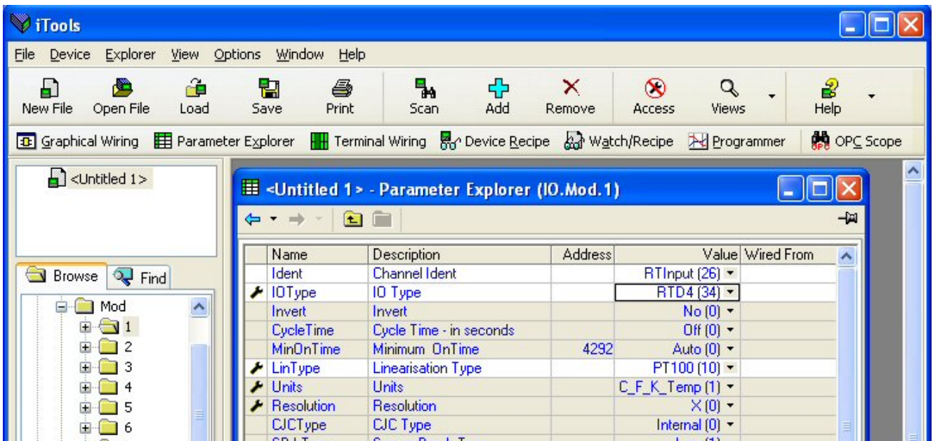
Figure 3-7: Module 1 defined as RTD4
