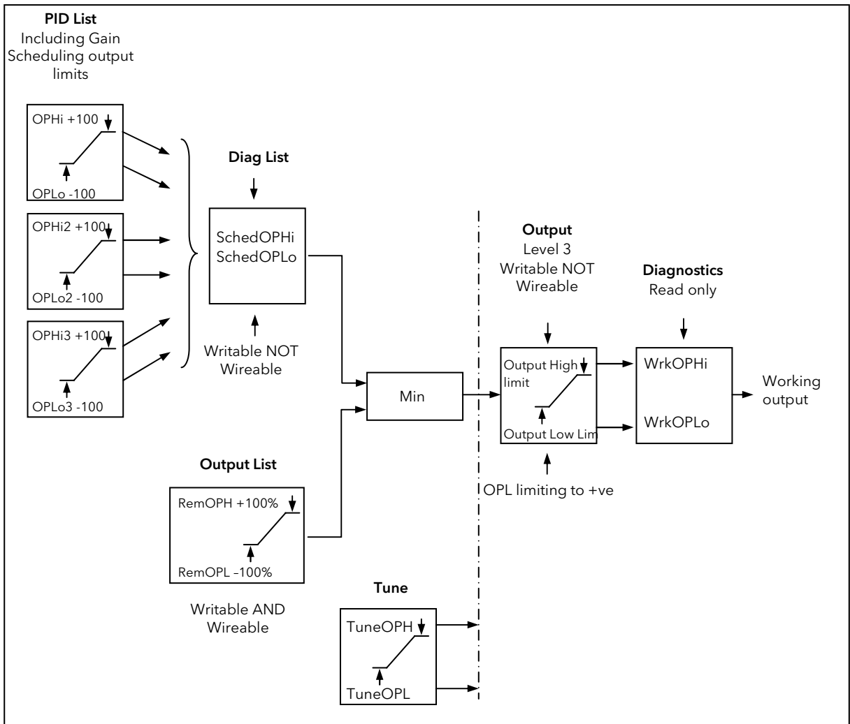
Figure 17-14: Output Limits
