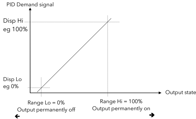
Figure 7-1: Time Proportioning Output
