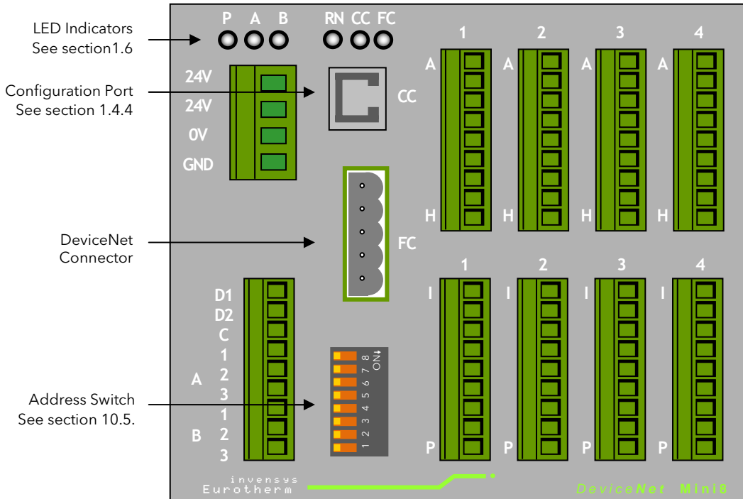
Figure 1-7: Front Panel Layout Devicenet
