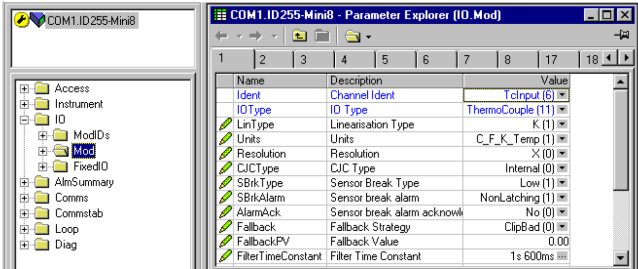
Figure 3-4: Thermocouple Input
