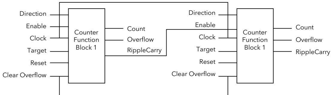
Figure 11-2: Cascading Counters
