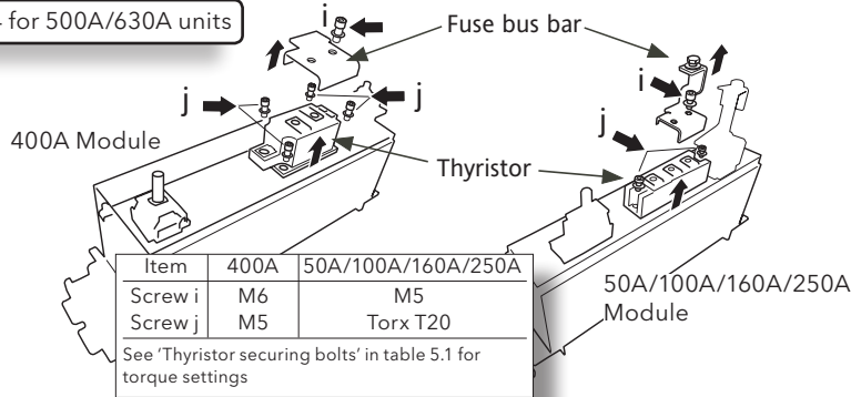
Figure 3.5 Thyristor removal (see section 4.4 for 500A/630A modules)
