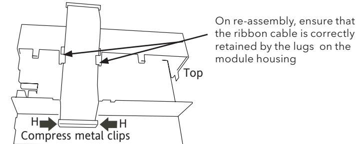
Figure 2.2.3 Ribbon cable
