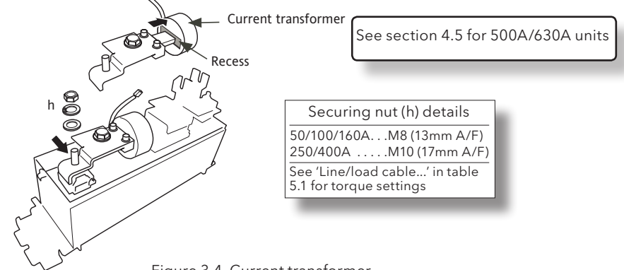
Figure 3.4 Current transformer (400A module shown; other modules similar but see section 4.5 for 500A/630A modules)
